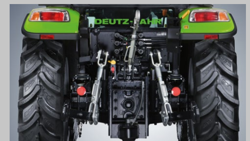
50 l/min hydraulic pump, up to three control valves, 3,500 kg rear power lift, 540/540ECO/1000 PTO.
